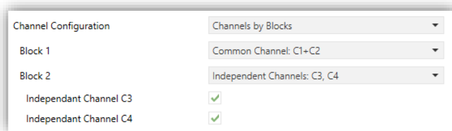
Figure 5 Channels by Blocks configuration in NarrowDIM X4.
