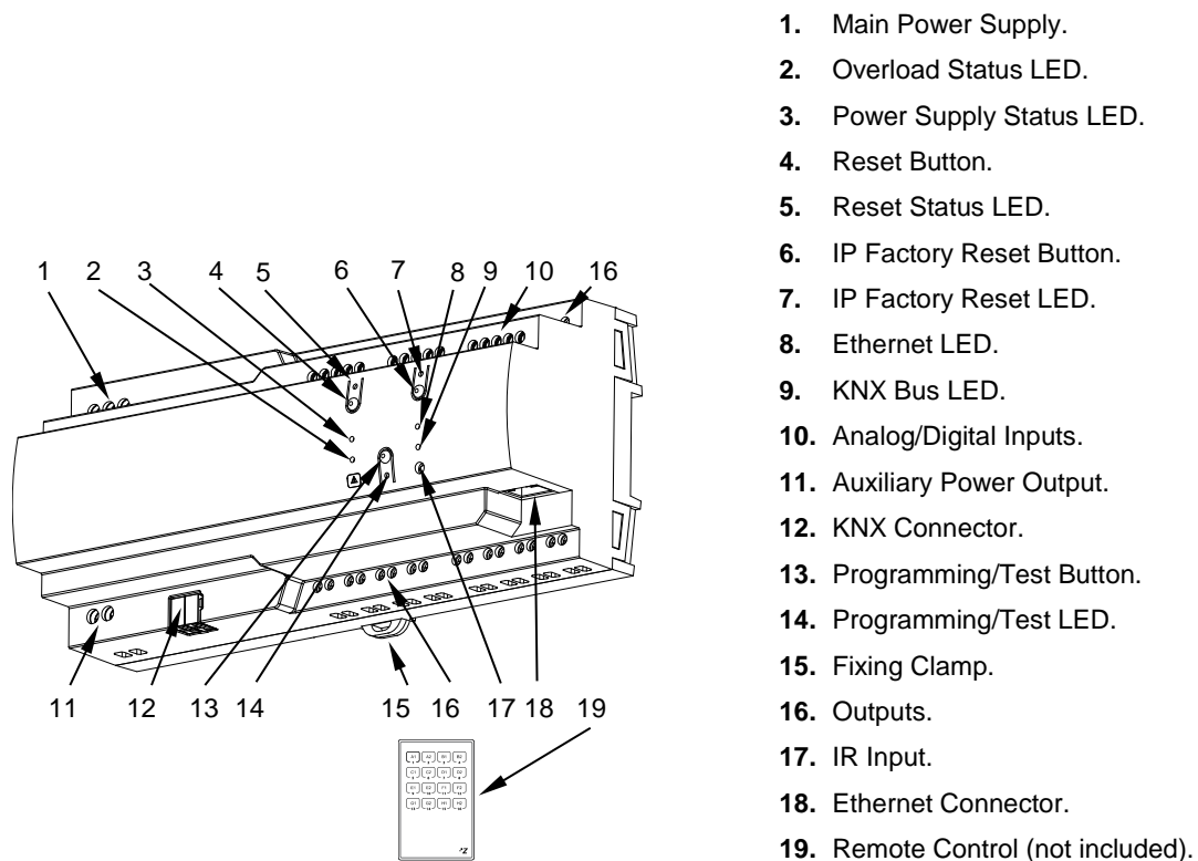
Figure 1. ALLinBOX 1612 v2 elements scheme.
