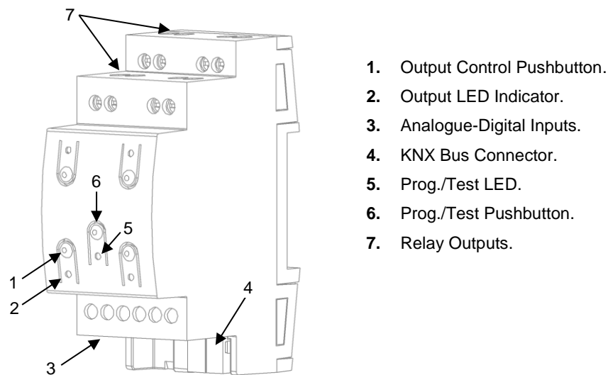
Figure 1. MINiBOX 45 v2. Elements
